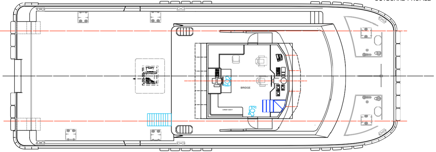
UPPER DECK PLAN
