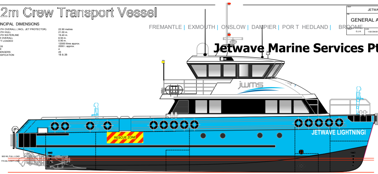
OUTBOARD PROFILE
